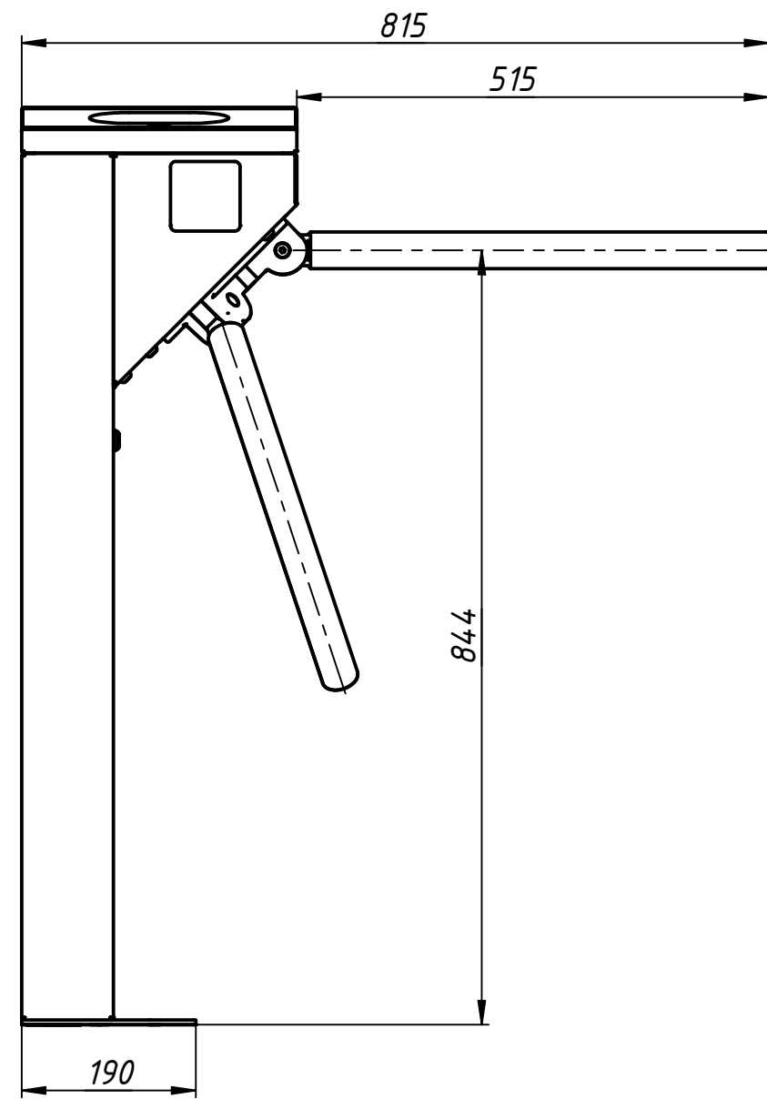
Installation tamplate
